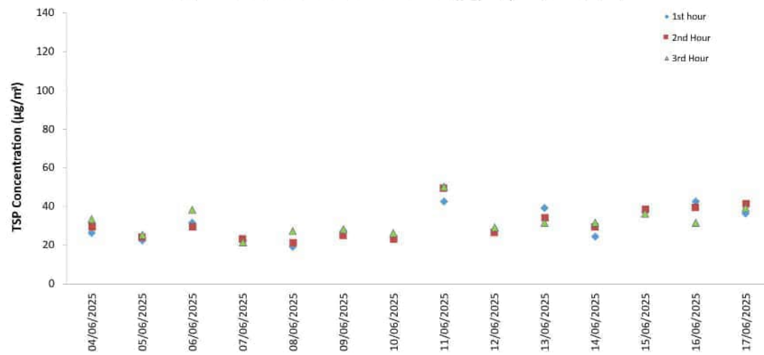
Measured 1-hour TSP Concentration ( \mu\text{g}/\text{m}^3 ) at Station AM1a
